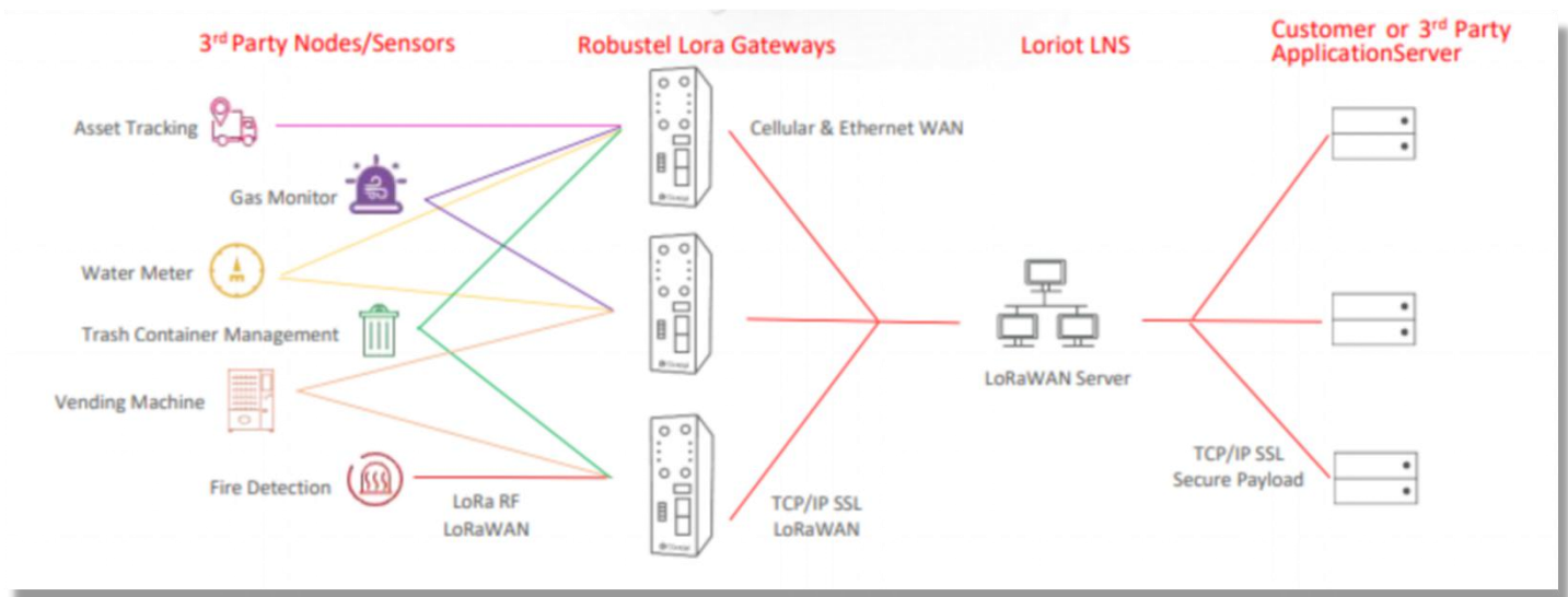
Figure 1.0 - “LoRaWAN stack enabled quickly & easily with the ‘Loriot APP’”
