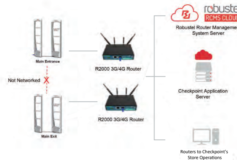
Figure 1.1 - Network topology of remote management solution
